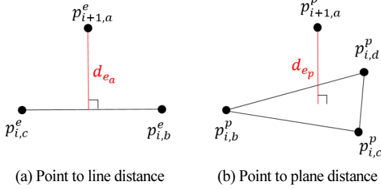
[Fig. 6] The feature points located at M_i form a line or plane, and calculate the distance from the feature points at K'_{i+1}(\lambda) . (a) p_{i+1,a}^e belongs to K'_{i+1}(\lambda) . p_{i,b}^e and p_{i,c}^e are feature points belonging to M_i^e . (b) p_{i+1,a}^p belongs to K'_{i+1}(\lambda) . p_{i,b}^p , p_{i,c}^p and p_{i,d}^p are feature points belonging to M_i^p
