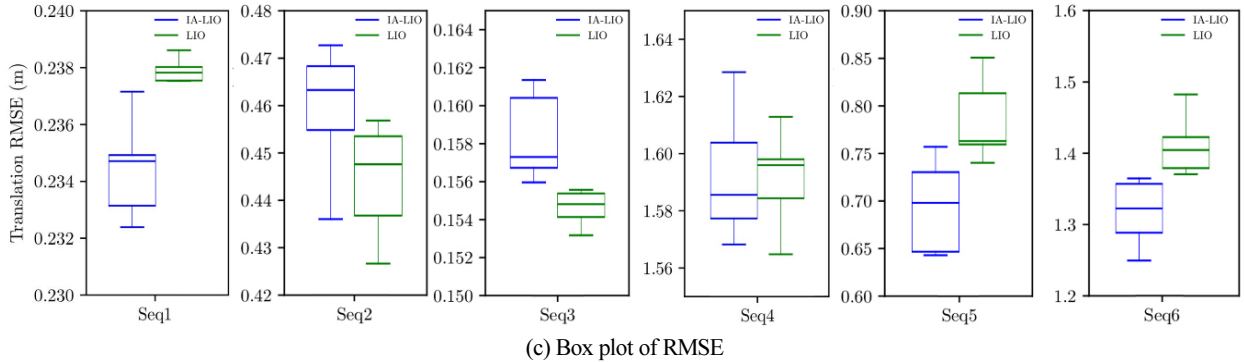
[Fig. 7] Result of dataset. (a) shows x-y trajectories of IA-LIO-SAM (blue), LIO-SAM (green), groundtruth (pink). Image below is the x-z trajectories. The real world image is shown in (b). Left image is top view of Seq 1 (red), Seq 2 (white), Seq 3 (blue). The top view of Seq 4 (blue region) and Seq 5,6 (red region).are in the middle image. In the right image, above is front view of Seq 4, and below is view of Seq 6 (also Seq 5). The result is shown in (c) through the box plot of RMSE
